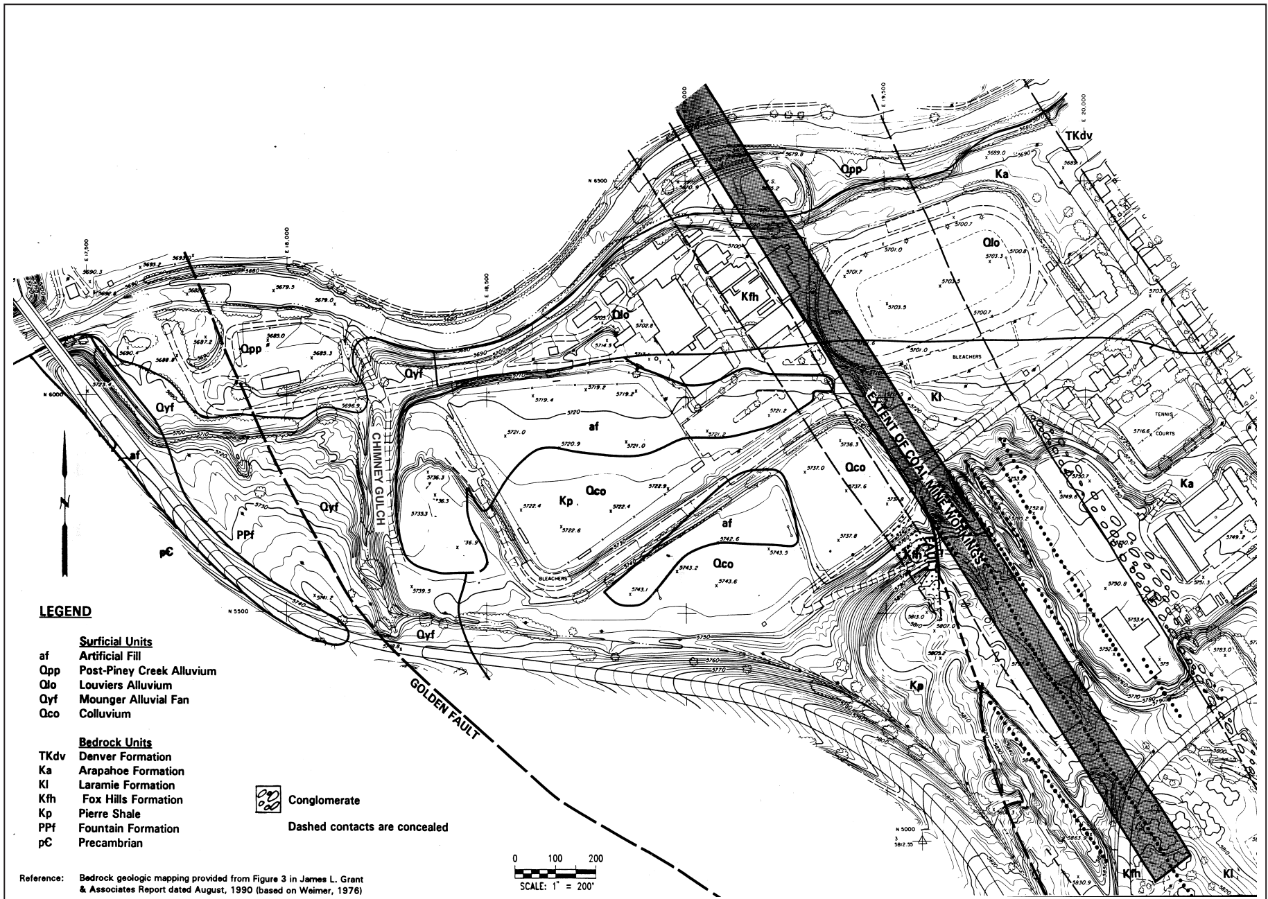
Figure 2-3 Area Surficial / Bedrock Geologic Map
