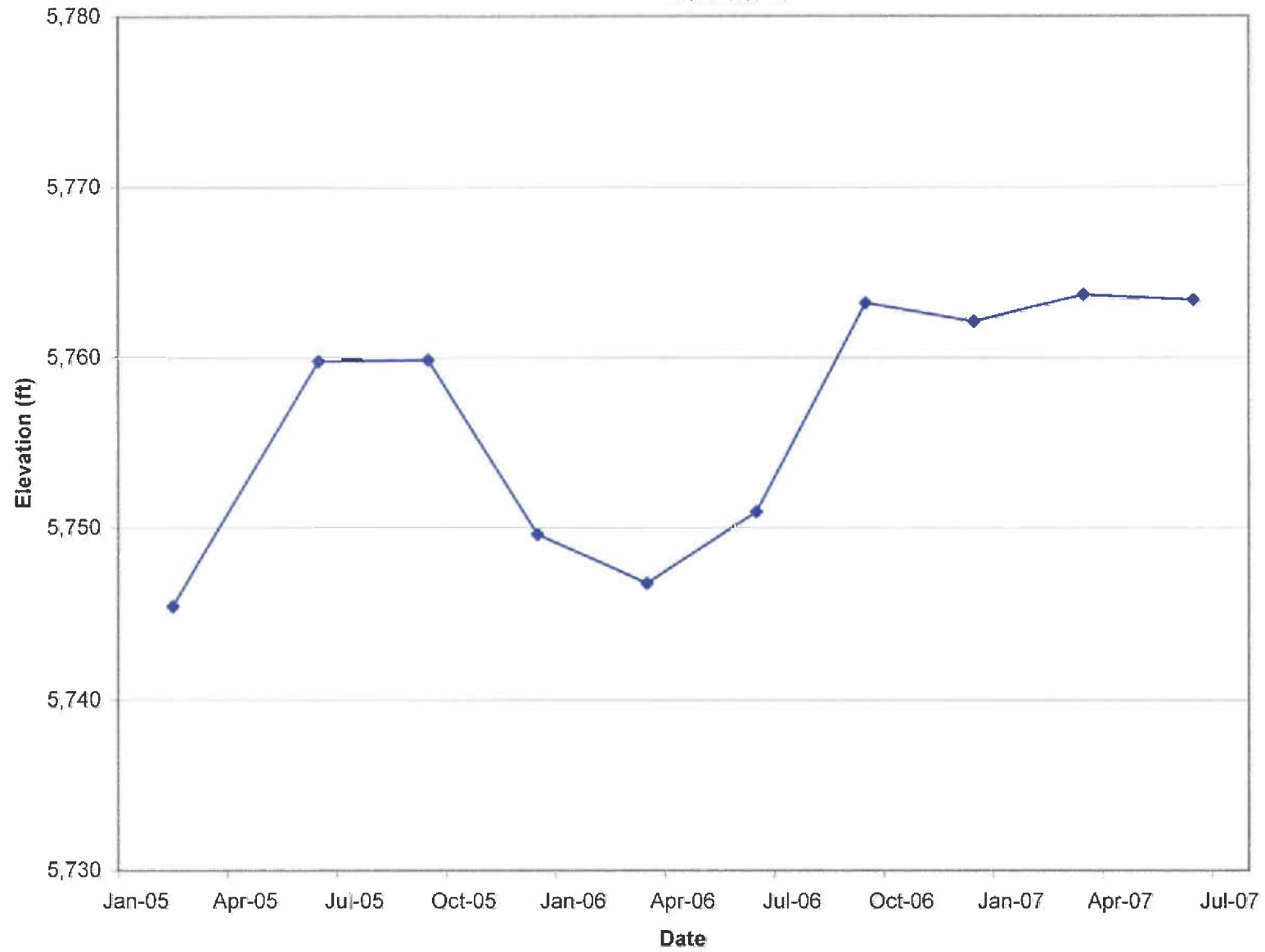
Figure 3 Hydrograph CSRMI-2
