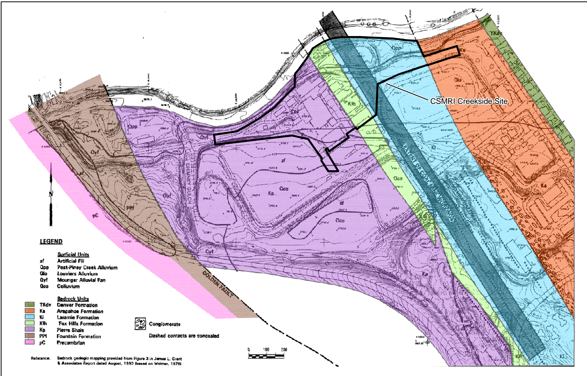
Figure 3 Bedrock Geologic Map of Site
